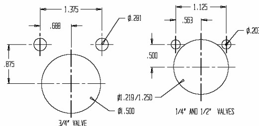
PANEL MOUNTED VALVE TEMPLATES
